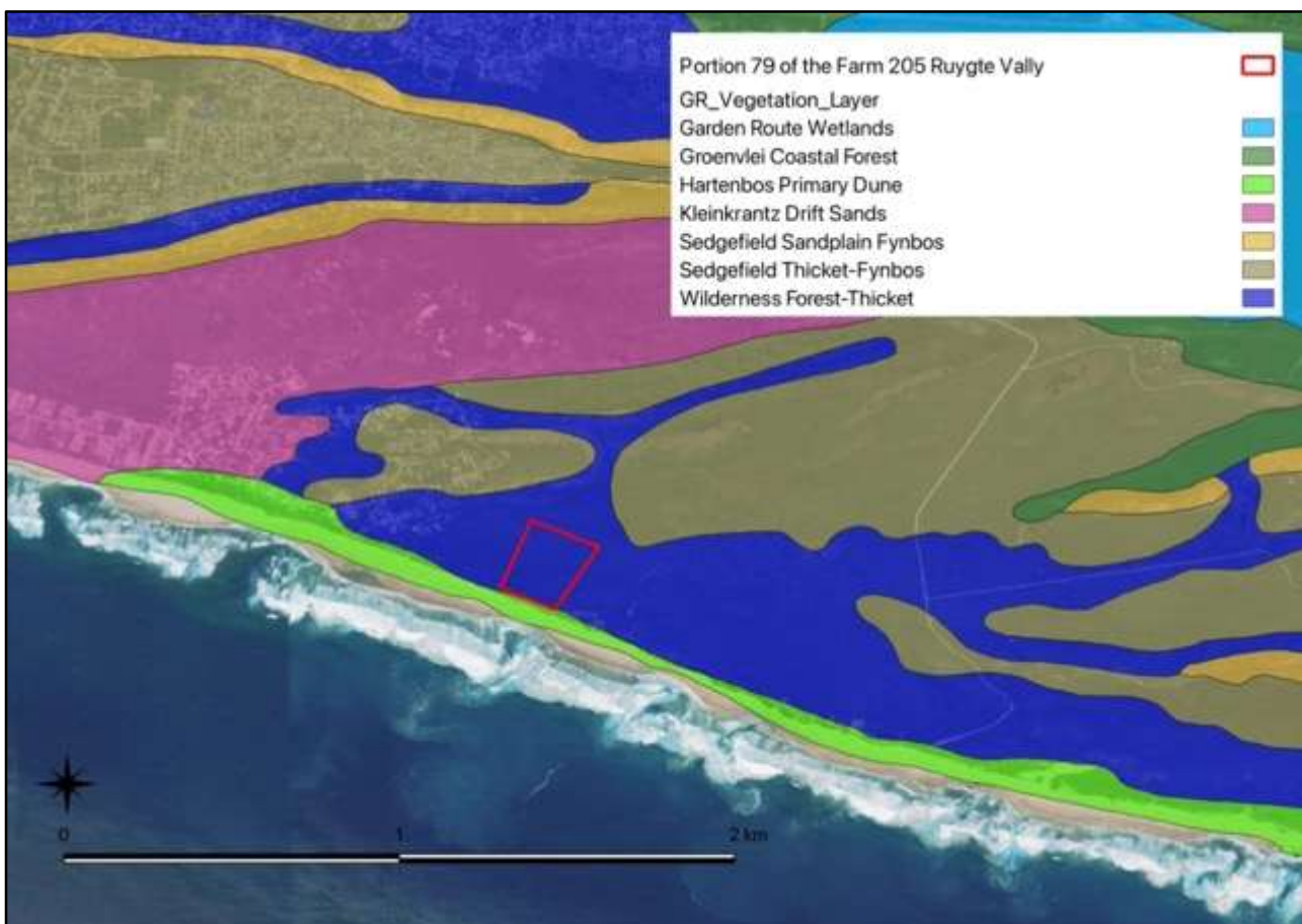
Figure 6: Vegetation types according to the Garden Route Initiative vegetation map.
