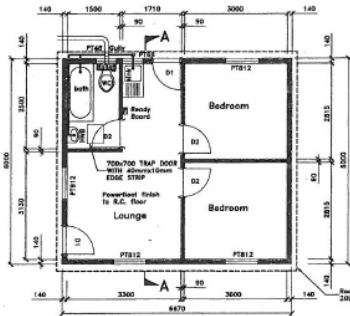
PLAN SCALE 1:50
