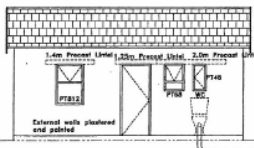
BACK ELEVATION SCALE 1:50
