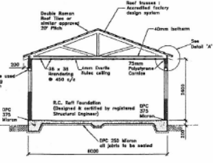
SECTION A-A SCALE 1:50
