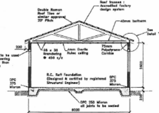
SECTION A-A SCALE 1:50
