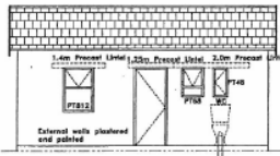
BACK ELEVATION SCALE 1:50
