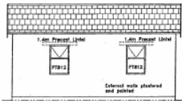
FRONT ELEVATION (Street Front) SCALE 1:50
